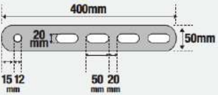
Forex 5mm | Diam. 300mm MG114.04
